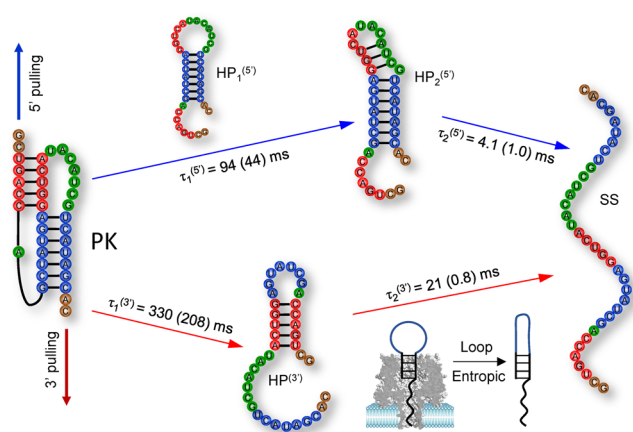
Figure 6. Predicted pathways of the nanopore unfolding of the T2 pseudoknot for the pulling from the 5' end (blue) and from the 3' end (red), respectively. Experimental dwell times and the mean first passage times (FPT) from KMC simulations (in parentheses) for the different steps are shown for comparison. The large difference of \tau_2^{(3')} (11 ms vs 0.8 ms) may be accounted for by the pausing time for the 8-nt loop in hairpin HP^{(3')} to overcome (mainly entropic) kinetic barrier to form compact conformations so HP^{(3')} can pass through the cis opening of the nanopore. In our model, we used g(V) = 1.8 \text{ kcal mol}^{-1} . Assuming g(V) = -Q_{\text{eff}}V as the electric potential-induced reduction in the energy barrier with V = 120 \text{ mV} for the potential drop across the nanopore in the experimental setup, we found the effective net charge Q_{\text{eff}} \approx 0.7 e for the chain inside the pore. 68 Noted that Q_{\text{eff}} is sensitive to the molecular types and the solution conditions, such as ion concentrations and pH value.
