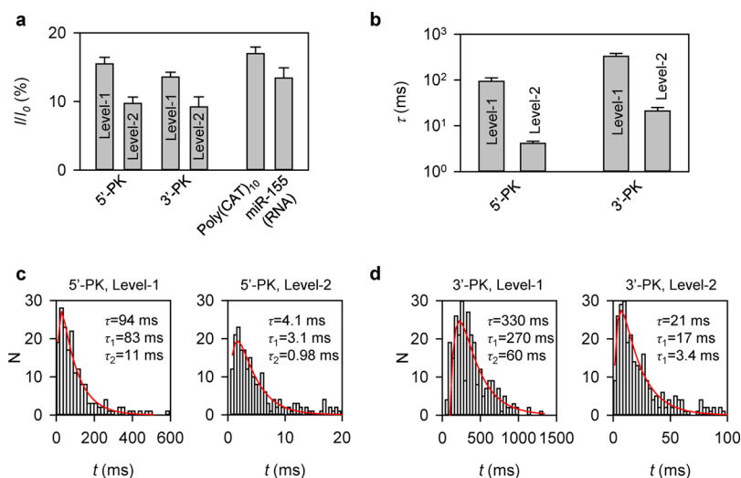
Figure 3. Characteristic blocking levels and durations of different steps in signatures of pseudoknots and control oligonucleotides. (a) Relative conductance ( I/I_0 , I and I_0 are current amplitudes of the block and empty pore) of Level-1 and Level-2 blocks in the 5'-PK and 3'-PK signatures shown in Figure 2b and c, and blocks generated by DNA Poly(CAT) 10 and RNA miR-155 translocation through the pore. Blocks of Poly(CAT) 10 and miR-155 were analyzed in Figure S3. (b) Durations of Level-1 and Level-2 stages in the 5'-PK and 3'-PK signatures. (c,d) Representative histograms of Level-1 (left) and Level-2 (right) durations for 5'-PK ( N = 245 ) (c) and 3'-PK ( N = 272 ) (d). The duration distributions in histograms were fitted with N(t) = A/(\tau_1 - \tau_2)[e^{-t/\tau_1} - e^{-t/\tau_2}] , based on a two-step kinetic pathway 111 (see Figure S10 for the fitting method). The duration of each level \tau was the sum of fitted \tau_1 and \tau_2 .
